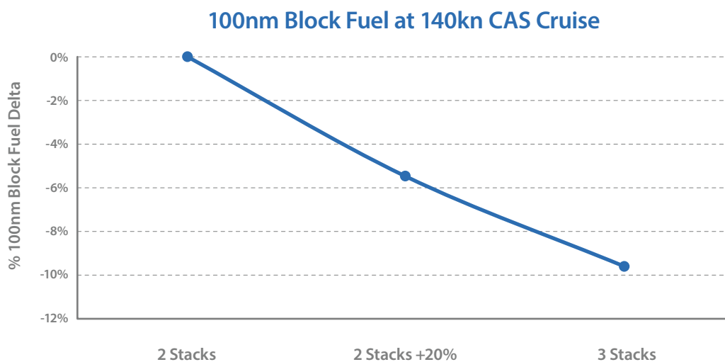
Figure 7 - Comparison of fuel cell stack size against block fuel
