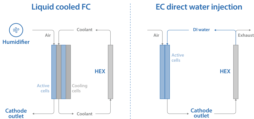
Figure 2 - Benefits of evaporatively cooled technology
