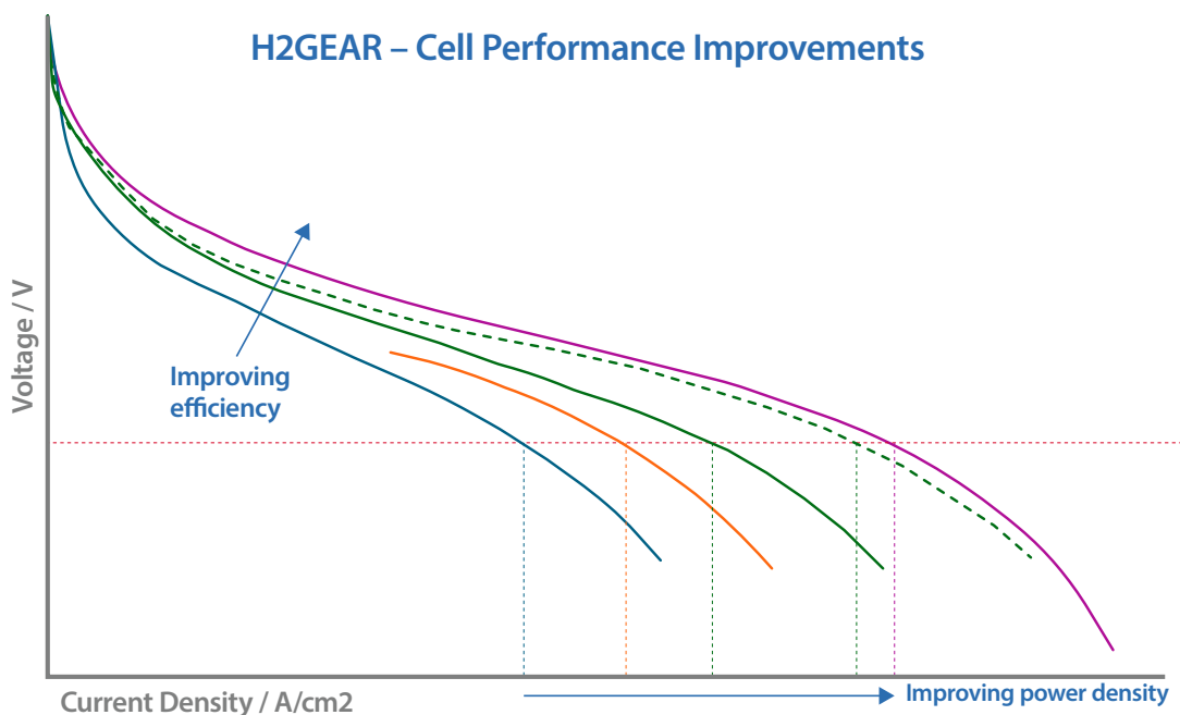
Figure 9 - Cell polarisation curve showing continuing performance improvements during H2GEAR
