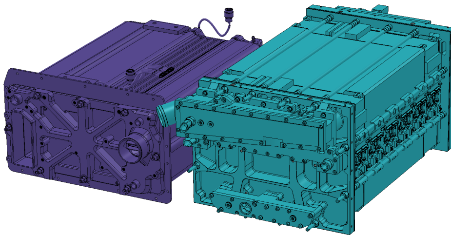
Figure 10 - Stack module developed under H2GEAR and size comparison with automotive stack
