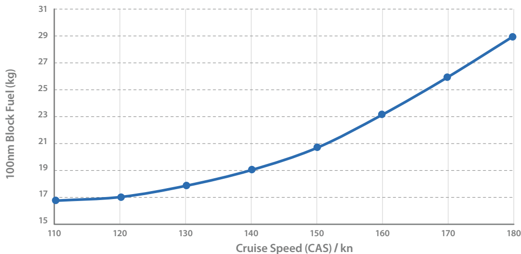
Figure 6 - Comparison of cruise speed against block fuel
