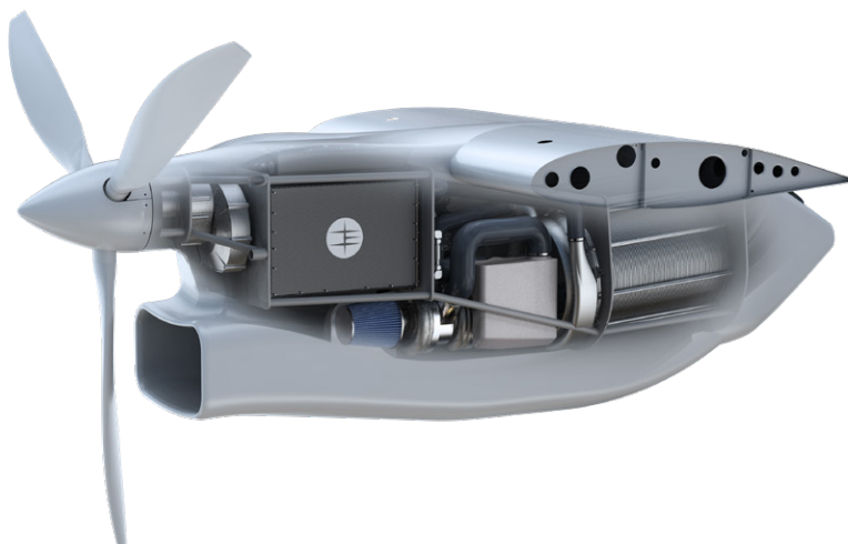
Figure 11 - Aircraft level integration of an EC hydrogen fuel cell system
